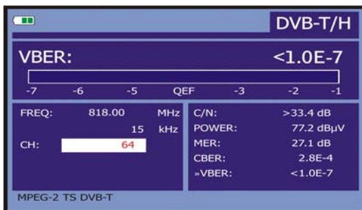
Figure 33.- DVB-T/H (COFDM) signals VBBER measurement screen.
